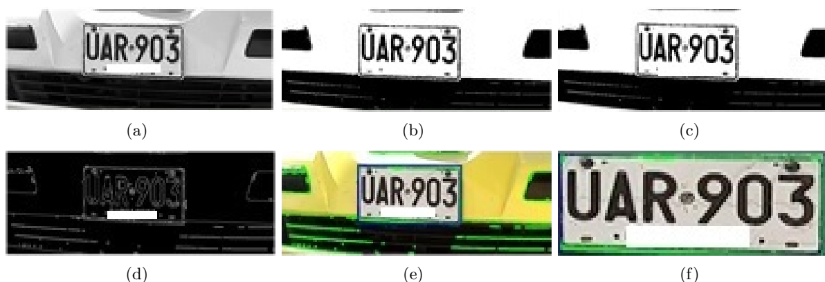
Figure 3. Segmentation process: (a) grayscale conversion, (b) binarization, (c) Gaussian blur, (d) edge detection, (e) identification of closed contours, (f) segmentation of the entire plate.
