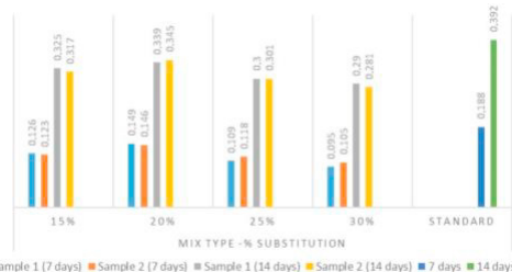
Fig. 2. Adhesive tensile strength (N) in mortars with corn husk ash.
