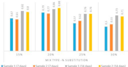
Fig. 4. Pozzolanic Activity Index in mortars with corn husk ash.
