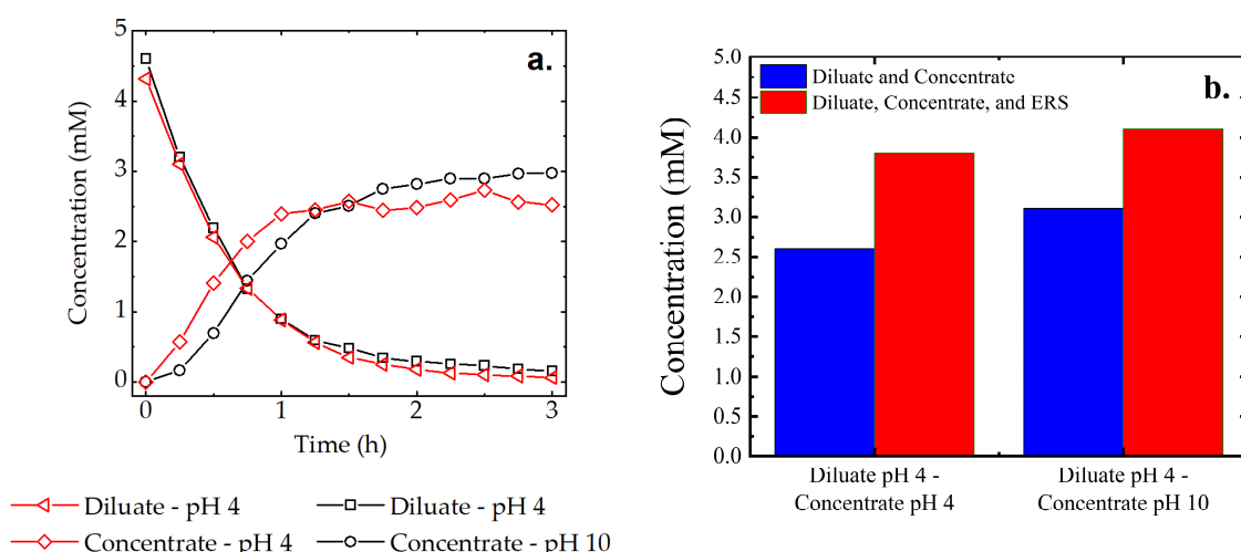
Figure 6. (a) Aniline concentration profiles in the diluate and concentrate channels during ED experiments. (b) Mass balances of aniline concentration in the diluate, concentrate, and ERS channels.
