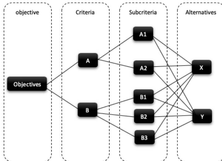
Figure 2. AHP process.
