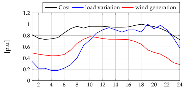
Figure A2. Input data for the numerical example.
