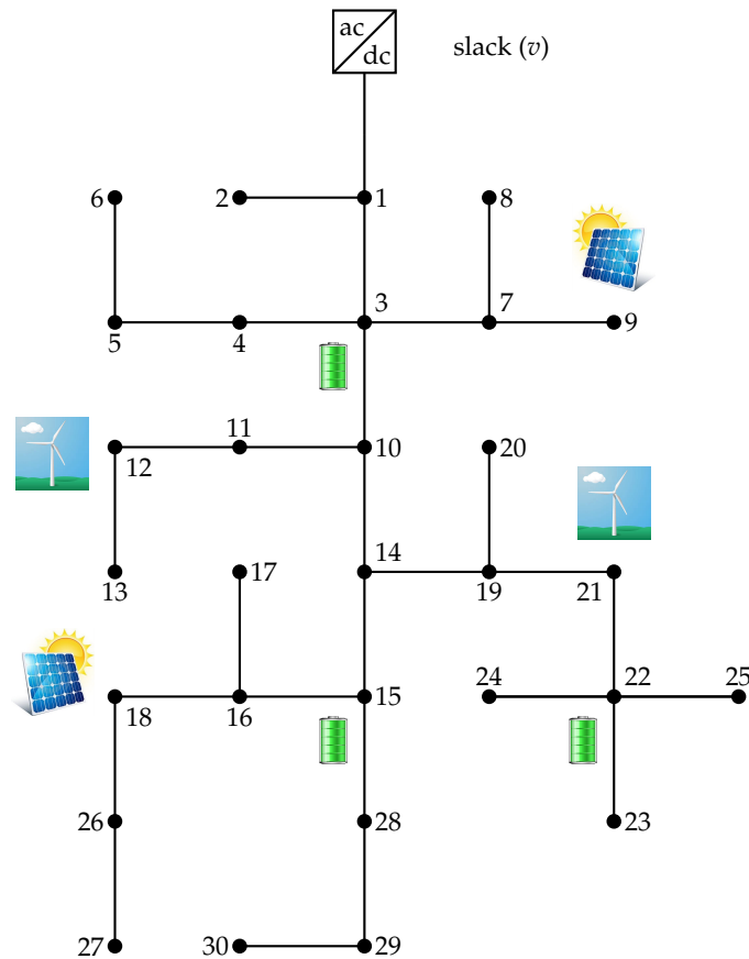
Figure 3. Electrical configuration of the 30-node test system.
