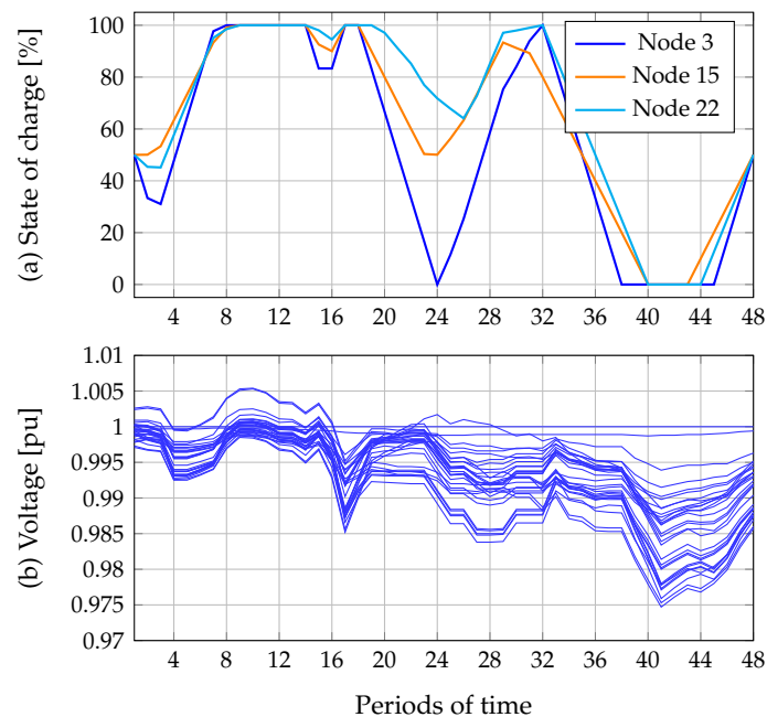
Figure 7. Batteries and voltage profile behaviors during a daily operation: (a) states of charge of each battery; and (b) voltage profiles in all the nodes.
