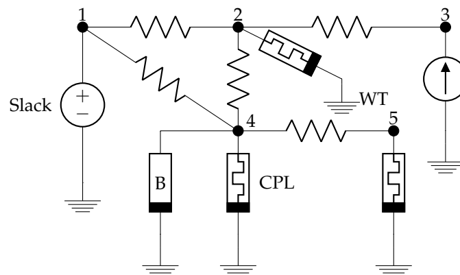
Figure A1. Grid connection for the numerical example.
