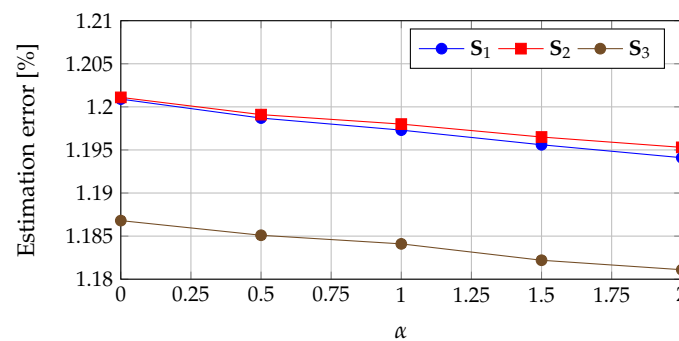
Figure 6. Final estimation error of the proposed artificial neural network for each load coefficient and operating scenario.
