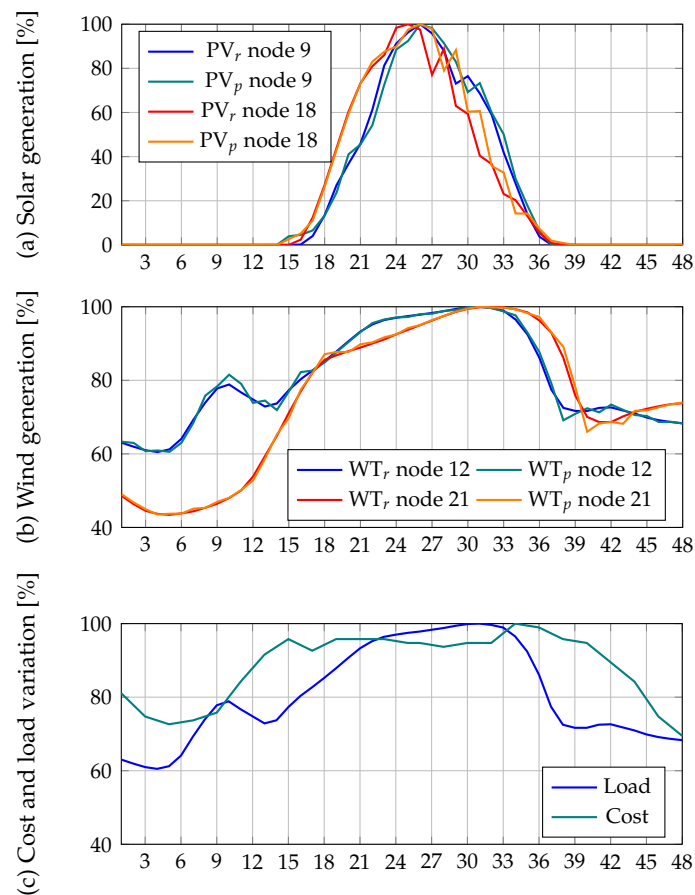
Figure 4. Behavior of renewable generation, demand, and costs during a daily operation: (a) real and predicted photovoltaic generation; (b) real and predicted wind generation; and (c) demand and cost behavior.
