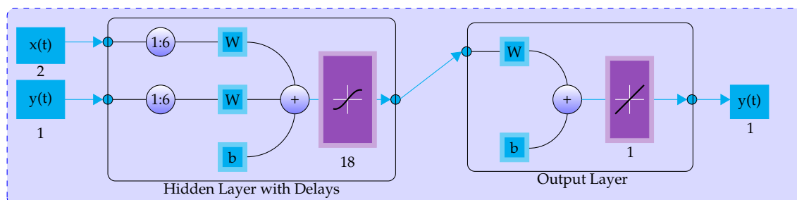
Figure 1. ANN for solar radiation prediction.
