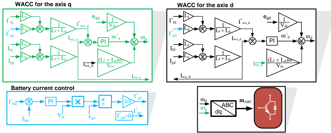
Figure 2. Scheme of the proposed WACC.
